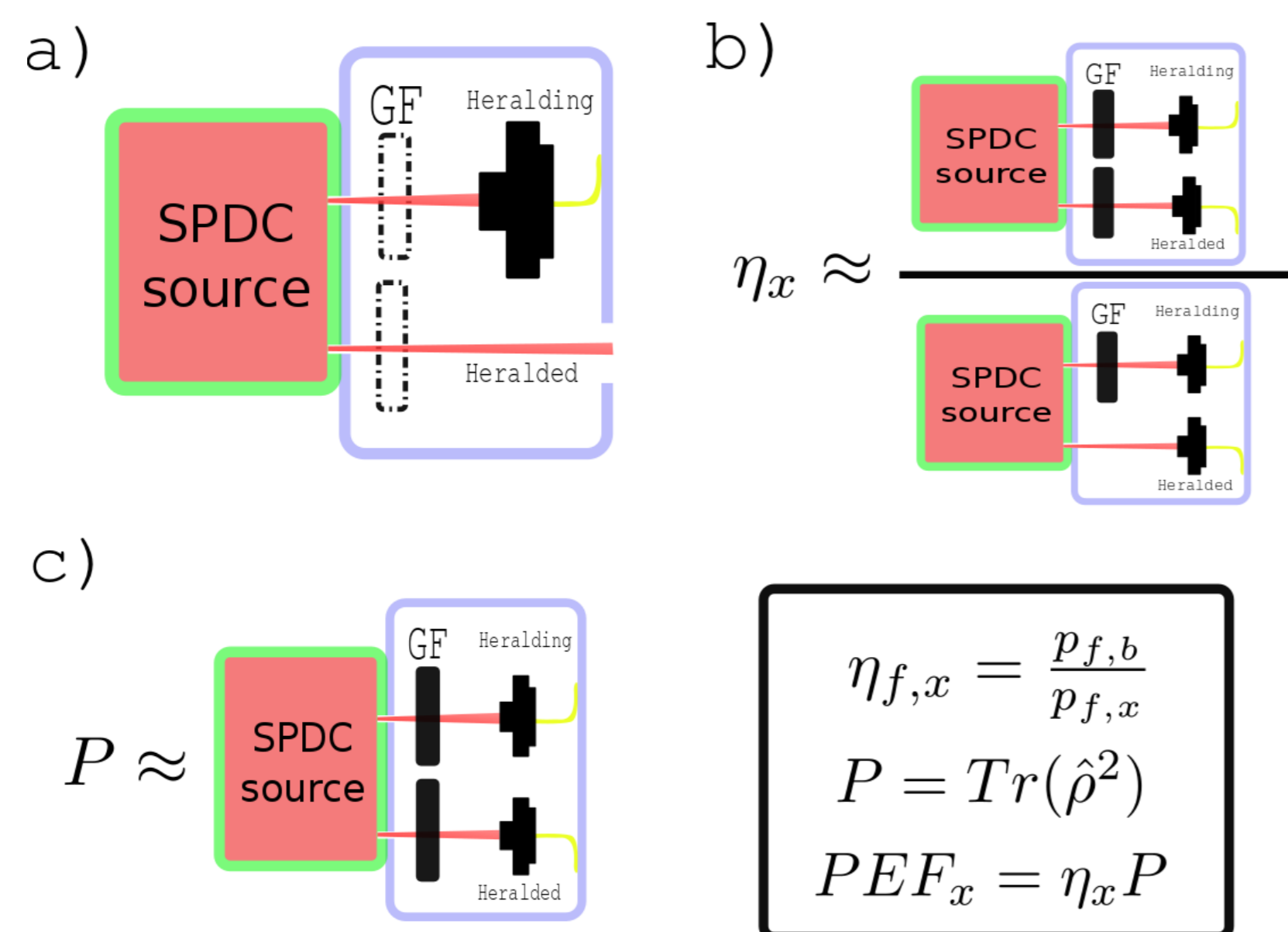
Figure 1: a) A heralding photon announces its partner. b) Heralded efficiency is proportional to joint detection with filters in both arms over the joint detection with a filter in the heralding arm. c) The purity is obtained by measuring the joint detection with spatial and spectral filters in both arms.
