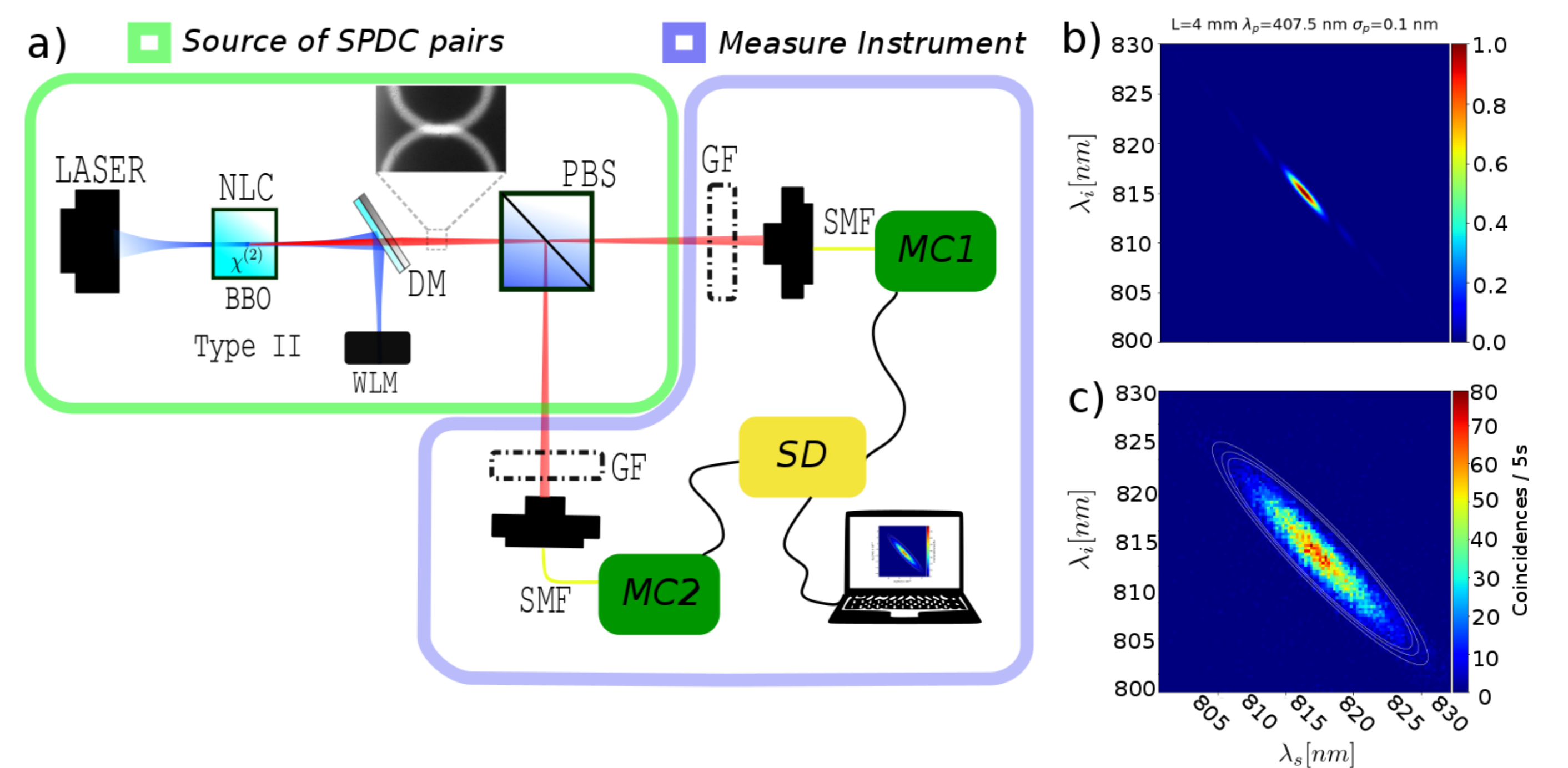
Figure 2: a) Experimental setup for the measurement of correlations between photon pairs produced by SPDC process. b) Theoretical and c) experimental measurement of the JS.
